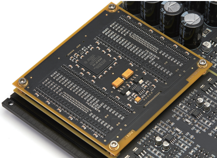
CYAN2 DAC Logic board
